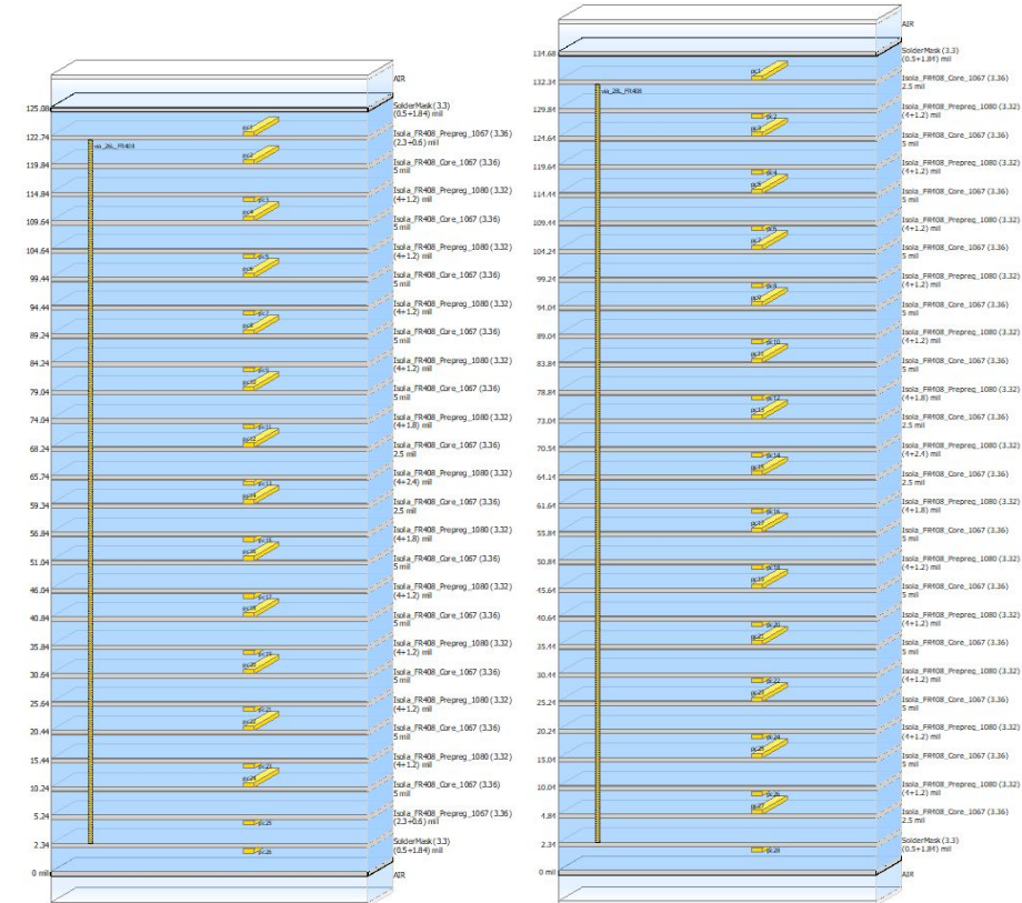
Figure A.12 - Definition of 26L PCB stack-up (left) and 28L PCB Stack-up (right)
