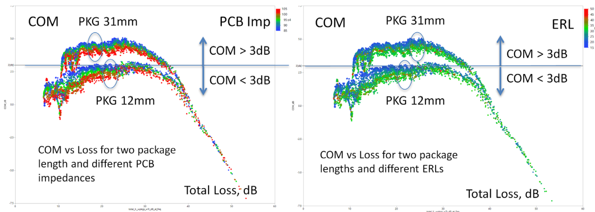
Fig. 6.8. COM vs link total loss at Nyquist frequency for two reference package lengths (12mm and 31mm, both graphs). Left graph shows PCB trace impedance in color from blue ( 85\Omega ) to red ( 105\Omega ). Right graph shows ERL coded in colors.
