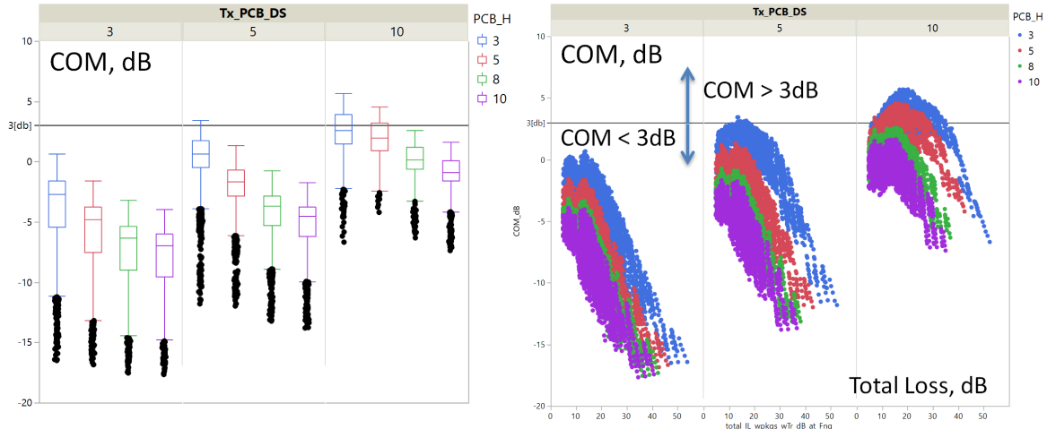
Fig. 7.5. Box plots for COM distributions (left graph) and COM vs link total loss at Nyquist frequency (right graph) for 4 dielectric thicknesses (coded with colors) and 3 pair to pair separations.
