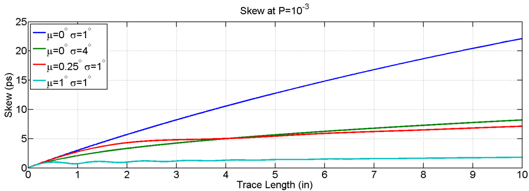
Figure 29: Skew at a failure threshold for four weave layers.
