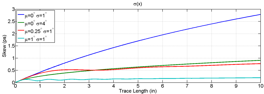
Figure 27: Skew standard deviation for various weave angle PDFs.
