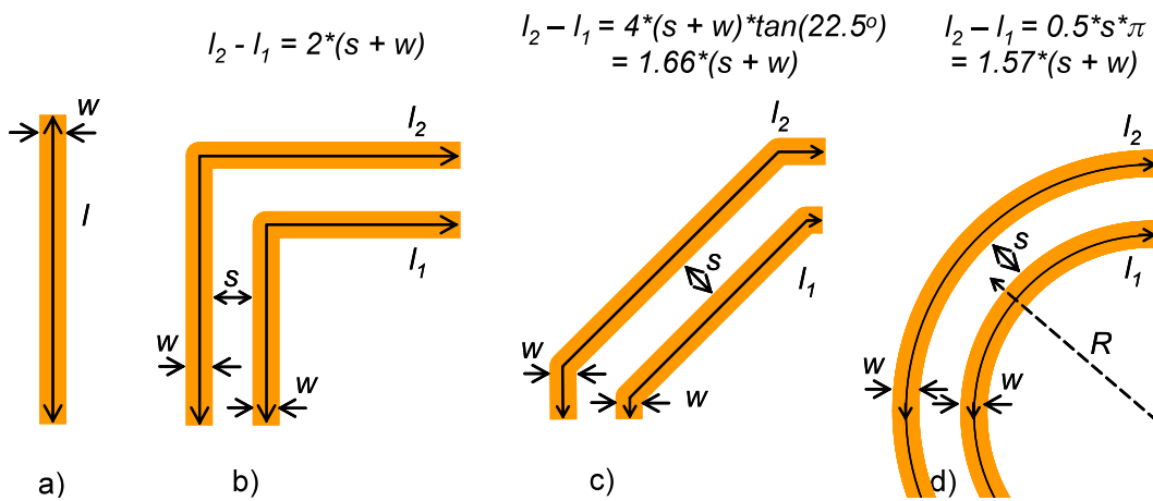
Figure 7: Center-line length differences of differential pairs based on layout geometry.
