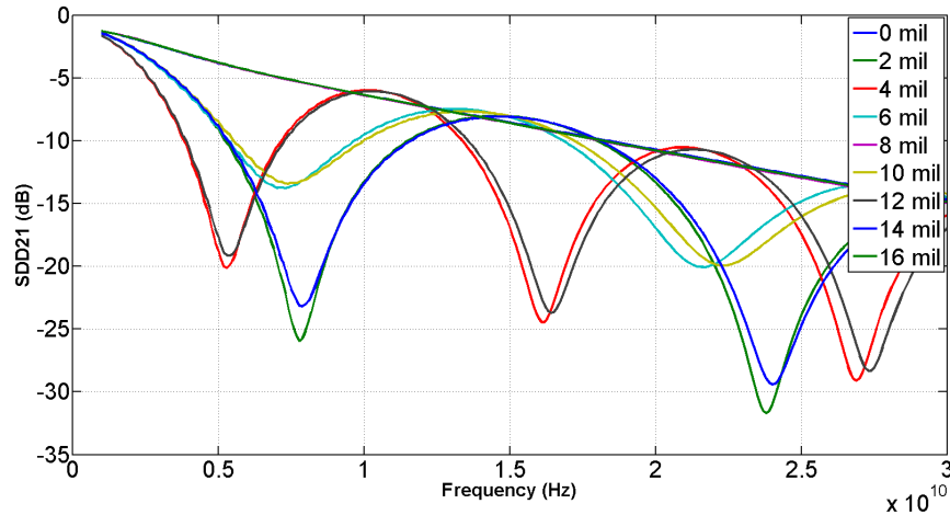
Figure 15: Skew resonances due to trace-3313 1-ply weave offset for 10 inches of stripline
