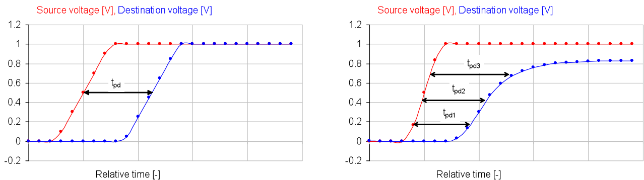
Figure 1: Illustration of delay definitions with ideal edges (on the left) and with different reference and target waveforms (on the right).
