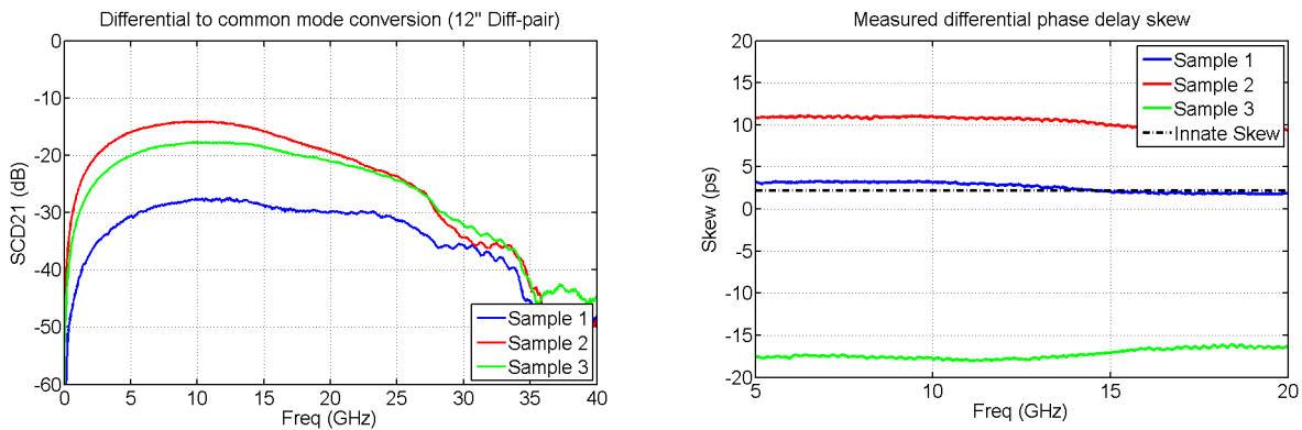
Figure 31: Mode conversion (left) and differential skew (right).
