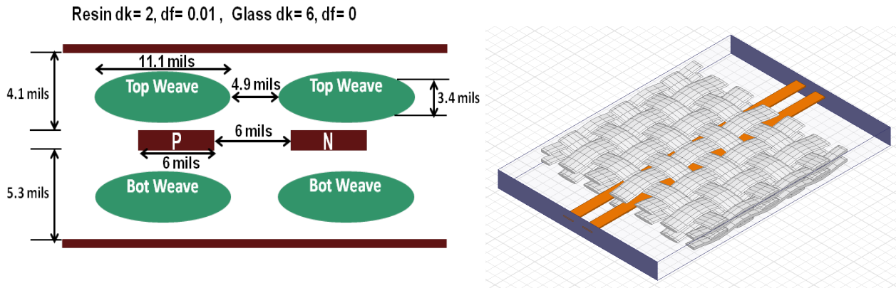
Figure 12: Geometrical description of the stripline structure with 3313 1-ply glass weave on top and bottom of the trace (left), 3D CAD stripline structure [10] with 3313 glass weave (on right)
