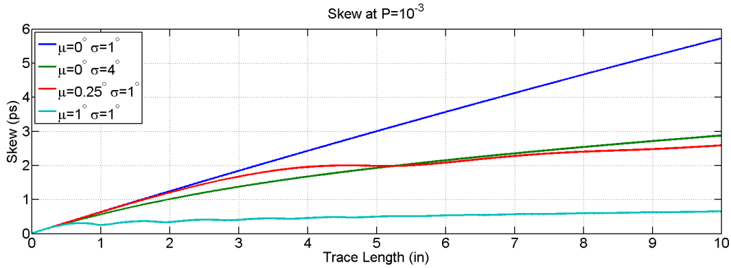
Figure 28: Skew at a failure threshold for a single weave layer.
