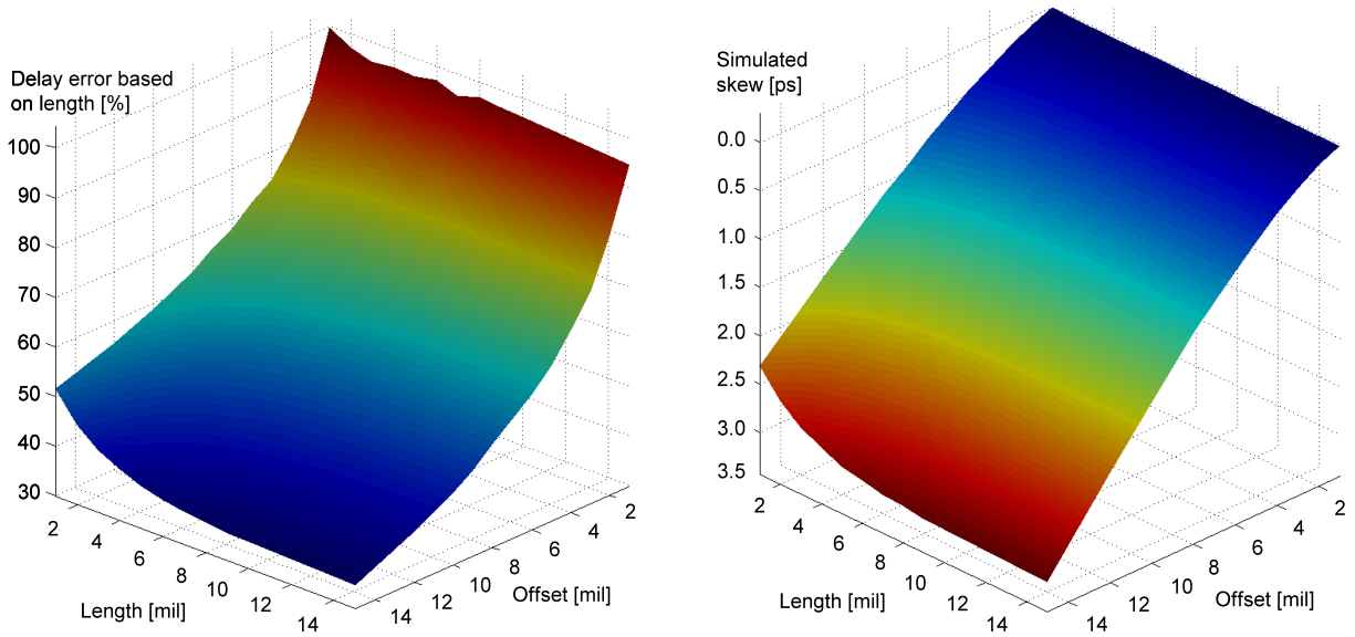
Figure 16: Calculated percentage skew error (on the left) and magnitude skew error (on the right) of a differential pair with a rectangular bulge on one leg, used for skew compensation.
