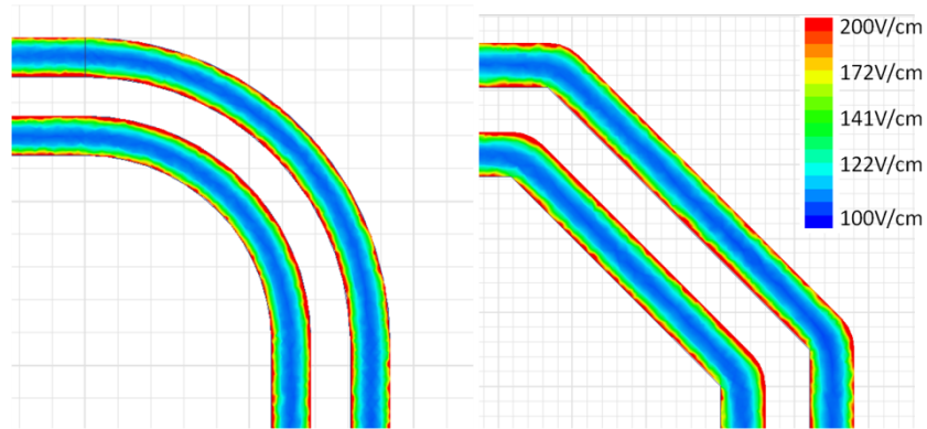
Figure 22: Surface current density at the different types of bends –arc (left) and double 45-degree (right).
