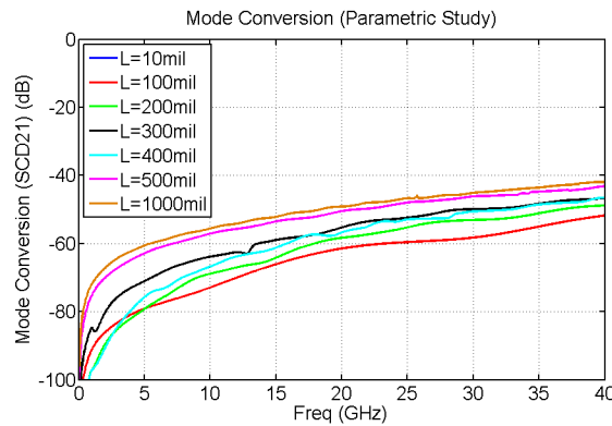
Figure 18: Differential to common mode conversion as spaces between trace bends changes.
