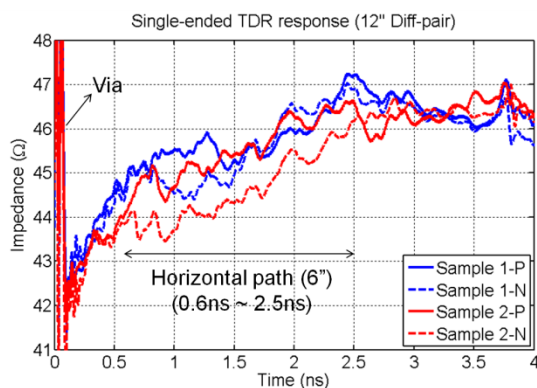
Figure 32: Calculated TDR response shows P/N impedance deviation.
