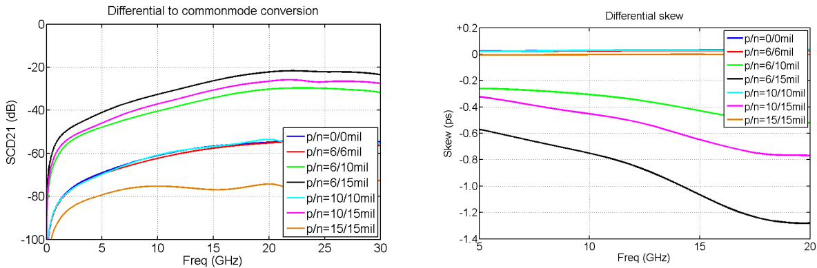
Figure 11: Differential to common mode conversion (left) and differential skew (right).
