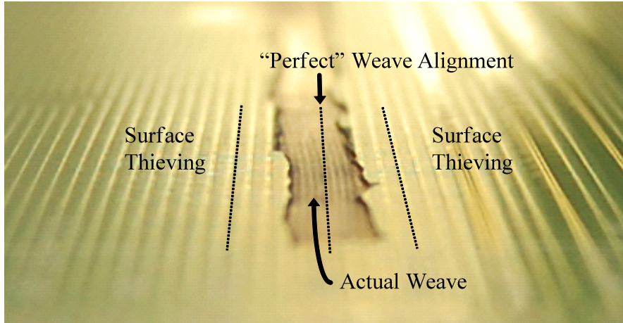
Figure 23: A partially milled PCB with weave that turns relative to surface thieving / panel edge. Image is taken at a shallow angle for contrast.
