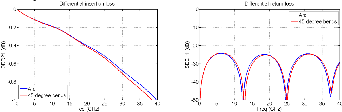
Figure 20: Differential insertion and return loss.
