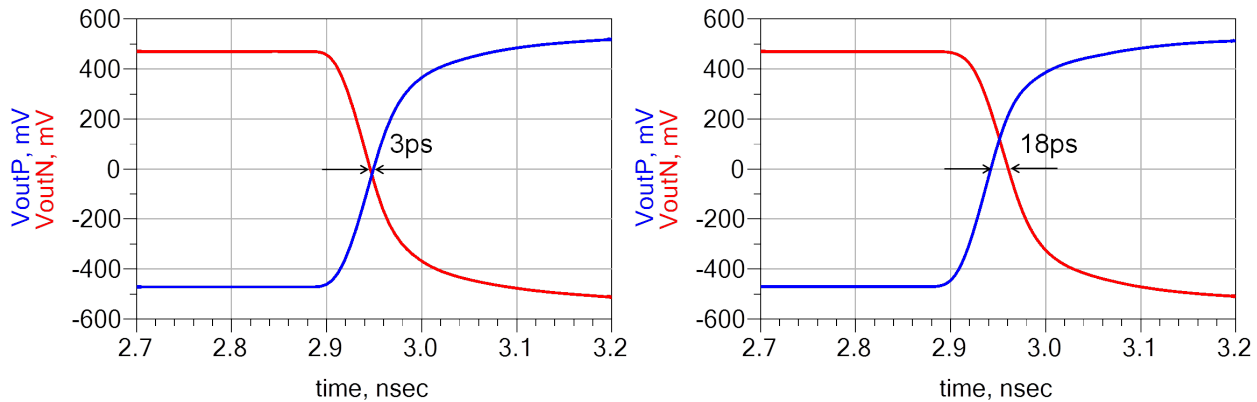
Figure 6: Distortion created by skew. Output voltages at the receiver show a difference between a board with 3ps (left) and 18ps (right) of skew.
