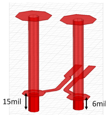
Figure 9: Asymmetric stub lengths
