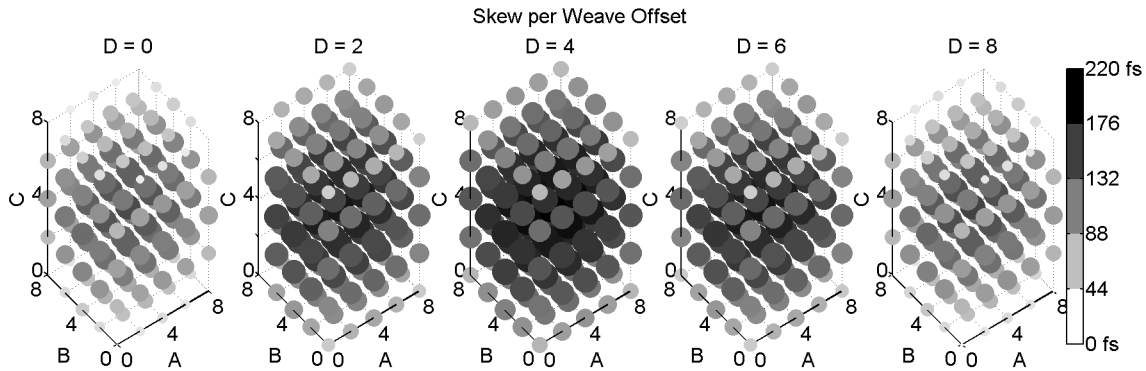
Figure 24: Skew at 10 GHz for 64 mils of differential etch, varied by weave offsets (A-D, mils).
