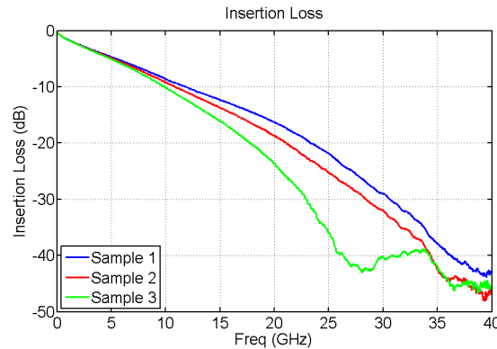
Figure 30: Differential insertion loss
