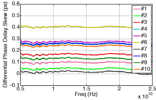
Figure 33: Differential phase delay skew error associated with cable movement and connector non-repeatability
