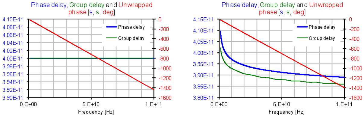
Figure 2: Phase delay and group delay for an ideal 50-ohm uniform transmission line (left) and a causal lossy 50-ohm transmission line of the same length (right).
