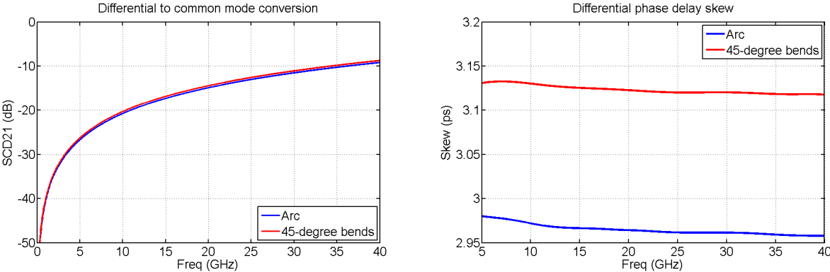
Figure 21: Differential to common mode conversion (left) and differential skew (right).
