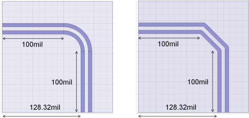
Figure 19: Two types of trace bends. An arc (left) and 45-degree bends (right).
