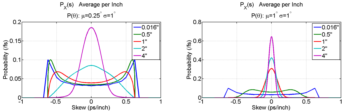
Figure 26: Skew PDFs for various weave angle PDFs.
