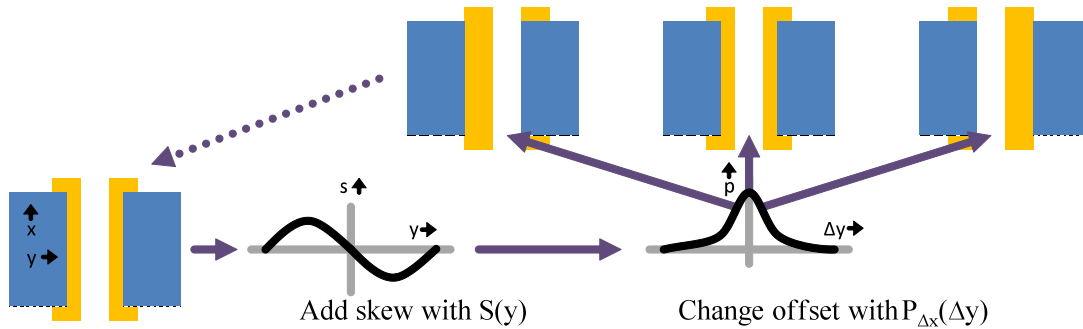
Figure 25: Steps for iteratively generating skew probabilities.
