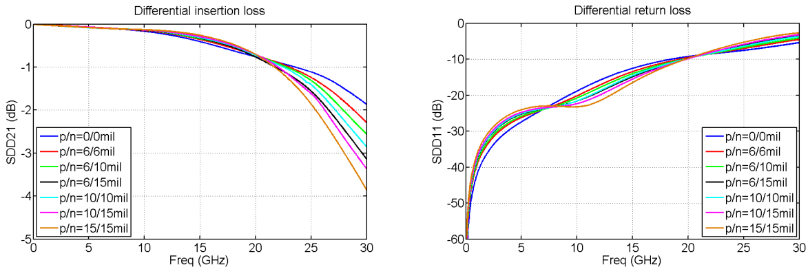
Figure 10: Differential insertion loss (left) and return loss (right).
