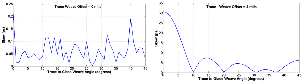
Figure 14: Impact of trace - 3313weave angle on skew for regular trace of 6 inches of stripline when the offset is 0 mils (on the left), and when the offset is 4 mils (on the right).
