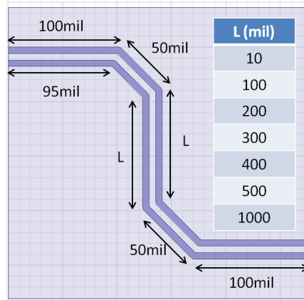
Figure 17: Differential pair with two 45-degree bends and the compensation bends.
