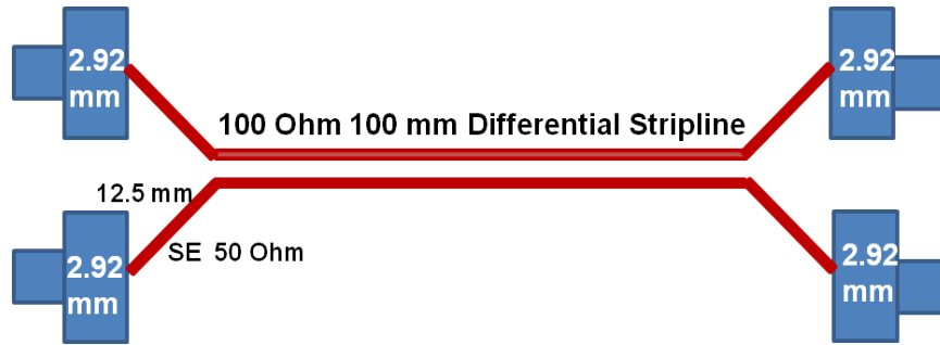
Figure 34: Geometry of the stripline surrounded by non-reinforced substrate.
