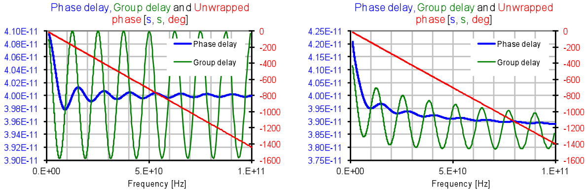
Figure 3: Phase delay and group delay calculated with 40-ohm reference impedance for an ideal 50-ohm uniform transmission line with 40 ps delay (left) and a causal lossy 50-ohm transmission line of the same length (right).
