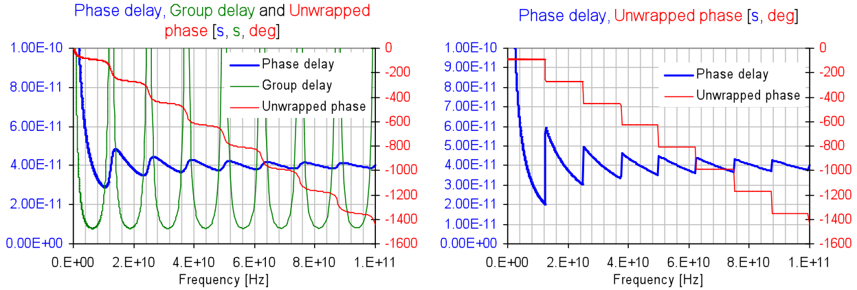
Figures 4 and 5: Phase delay and group delay calculated with 500-ohm reference impedance (on the left) and 500 kOhm reference impedance (on the right) for an ideal 50-ohm uniform transmission line with 40 ps delay.
