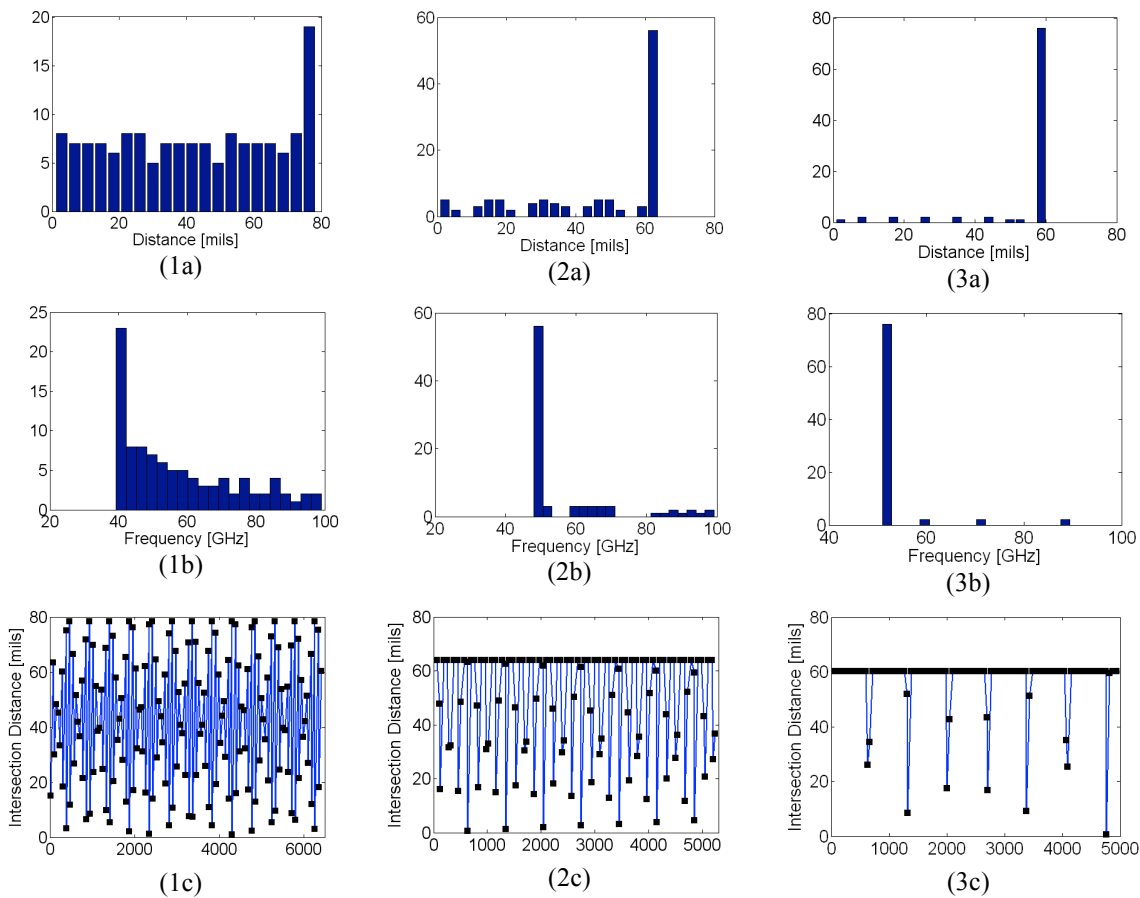
Figure 10 Row (a): Histograms of the distance between neighboring intersections for a trace route angle of 50 (1a), 70 (2a), and 85 (3a) degrees. Row (b): Histograms of the equivalent SCP frequency for a route angle of 50 (1b), 70 (2b), and 85 (3b) degrees. Row (c): Intersection distances as you move along the trace path for the 50 (1c), 70 (2c) and 85 (3c) degree routes. The x-axis shows the number of intersections, not the length of the trace.
