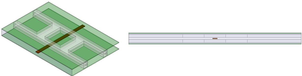
Figure 1 Left: Idealized stripline structure showing the glass weave pattern. For the glass, D_k and D_f were 6 and 0%, respectively. For the resin, D_k and D_f were 3.5 and 3%, respectively. The total trace length was 5 inches. Right: Cross-sectional view of the structure. The dielectric thickness above and below the trace remained constant at 4 mils. Each glass layer (nominally 3 mils thick) was centered symmetrically in the resin, on both sides of the trace, offset by 0.5 mils.
