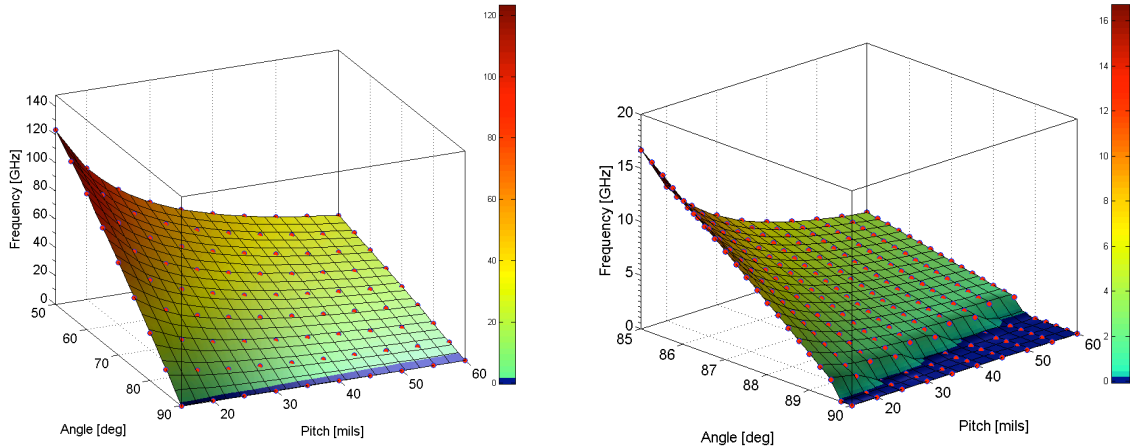
Figure 12 Surface plot of the MCP resonance frequency for a 2500 mil trace routed at 50-90 degrees ( left ) and a more detailed simulation run focusing on 85-90 degrees ( right ) using glass-weave pitches ranging from 15-60 mils. The red dots are simulated values whereas the surface is interpolated.
