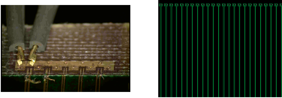
Figure 16 Left : Photograph of the top end of the traces showing the wafer probe used for the measurements. Right : Snapshot of the board layout showing the wide array of trace pitches and widths that were measured.
