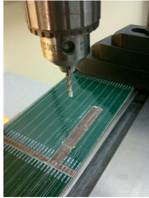
Figure 20 Photograph of the milling machine and secured board. Careful adjustments and measures were taken which allowed the board to be milled in approximately one-mil increments.
