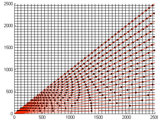
Figure 11 Example of glass-weave grid (black) with overlaid traces (red) at 2.5 degree steps. Only horizontal glass bundle crossings are shown. The grid pitch is 60 mils. The units are in mils.
